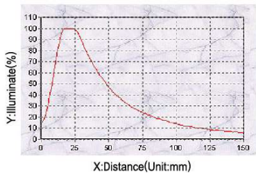
GL-DR6736R Graph
